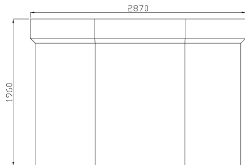
Inlet Elevation
